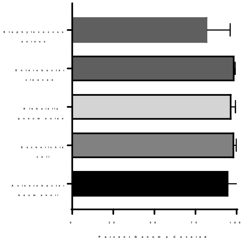
Genome coverage achieved
